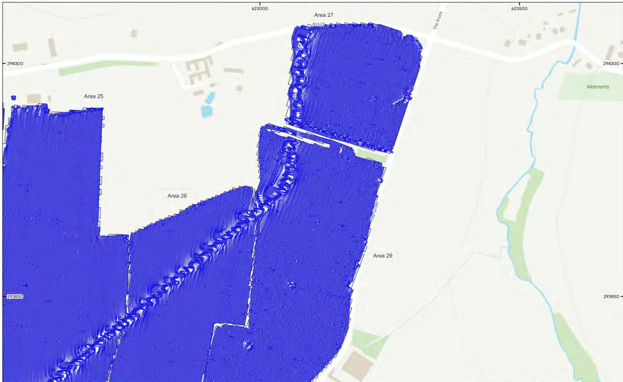
MSTM1774 - East Pye Solar Farm Figure 115 - XY Plot (Areas 25, 26, 27 & 29) 180nT/cm at 1:3,000 @ A3 © Magnitude Surveys 2025 Contains Ordnance Survey data © Crown Copyright and database right 2025
