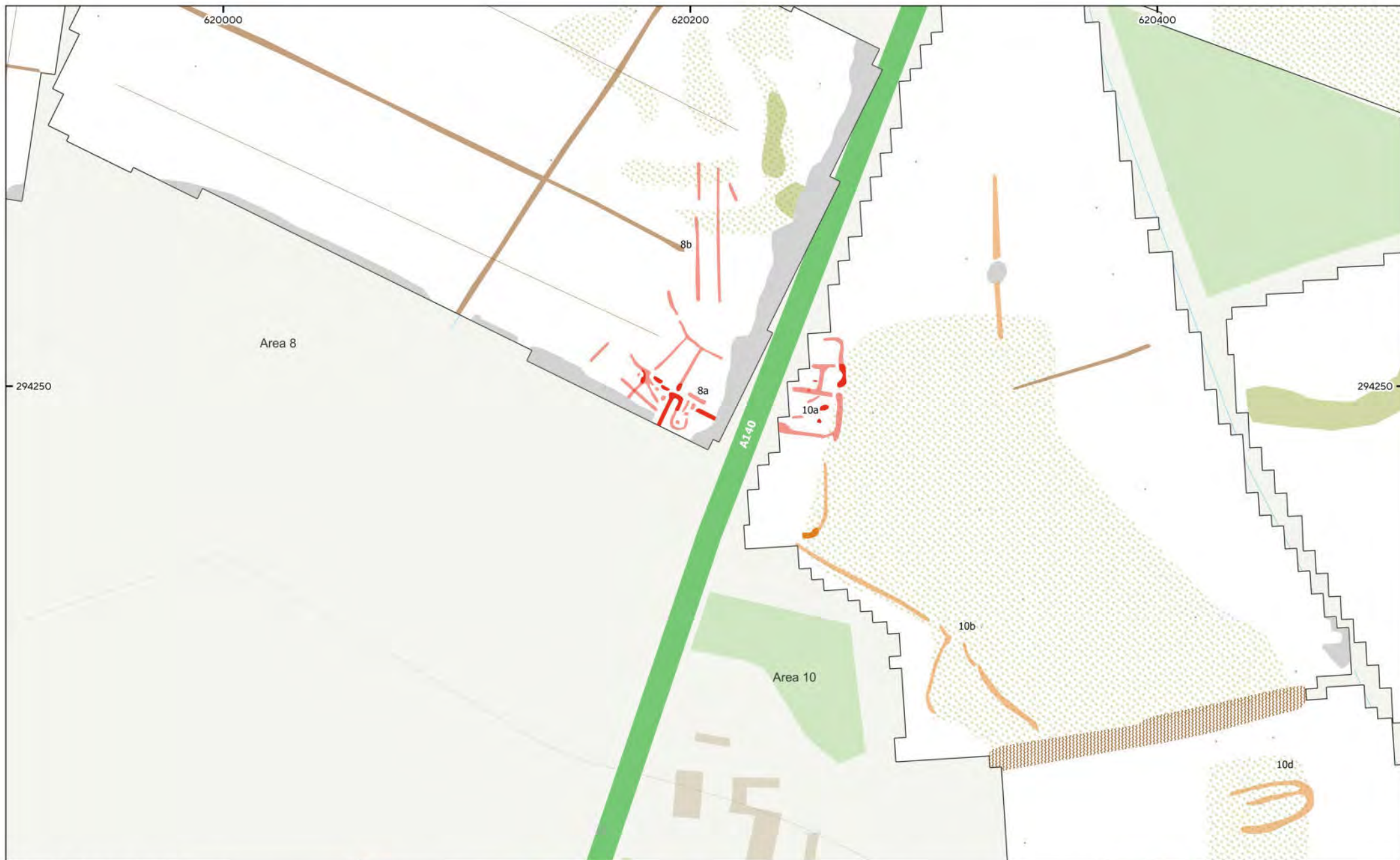
MSTM1774 - East Pye Solar Farm Figure 189 - Magnetic Interpretation (Area of Archaeological Activity 1 (Areas 8 & 10)) 1:1,500 @ A3 © Magnitude Surveys 2025 Contains Ordnance Survey data © Crown Copyright and database right 2025
