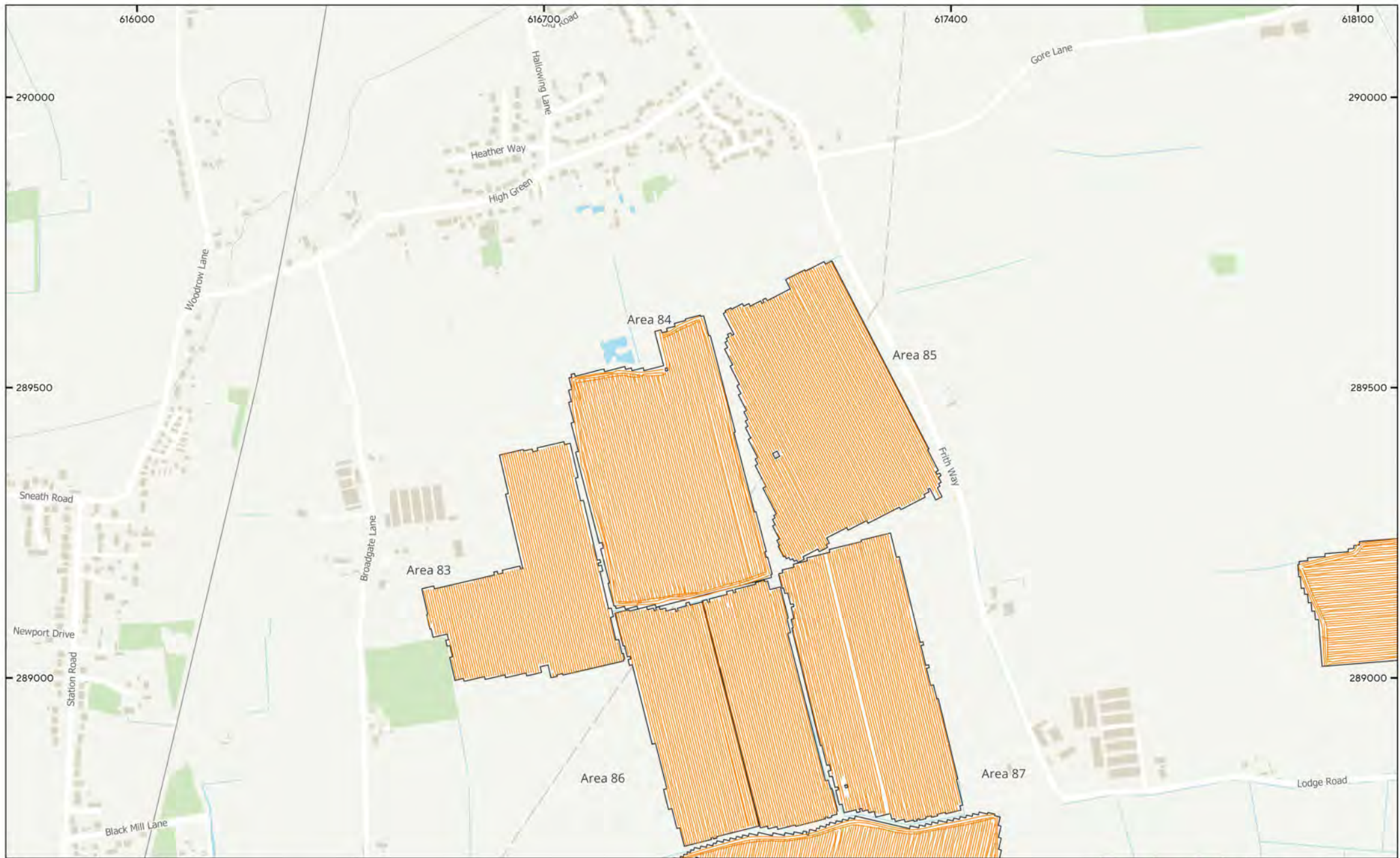
MSTM1774 - East Pye Solar Farm Figure 7 - GNSS Plot (Site 1 (Areas 2 & 82 to 87)) 1:6,000 @ A3
