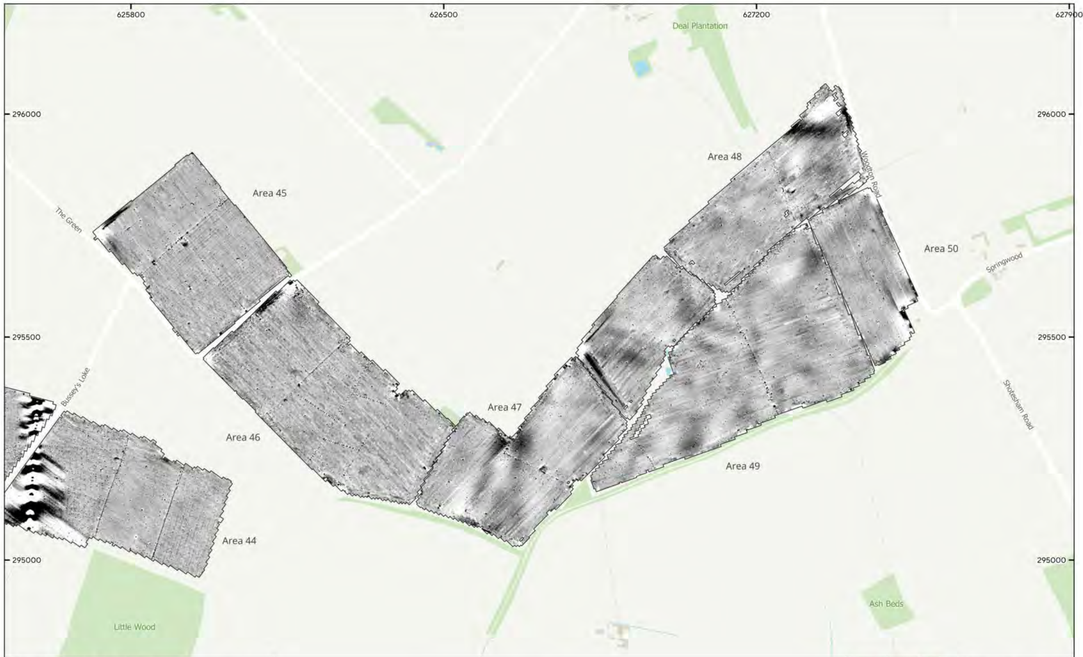
MSTM1774 - East Pye Solar Farm Figure 35 - Magnetic Total Field Overview (Site 7 (East) (Areas 44 & 45 to 50)) 1:6,000 @ A3 © Magnitude Surveys 2025 Contains Ordnance Survey data © Crown Copyright and database right 2025
