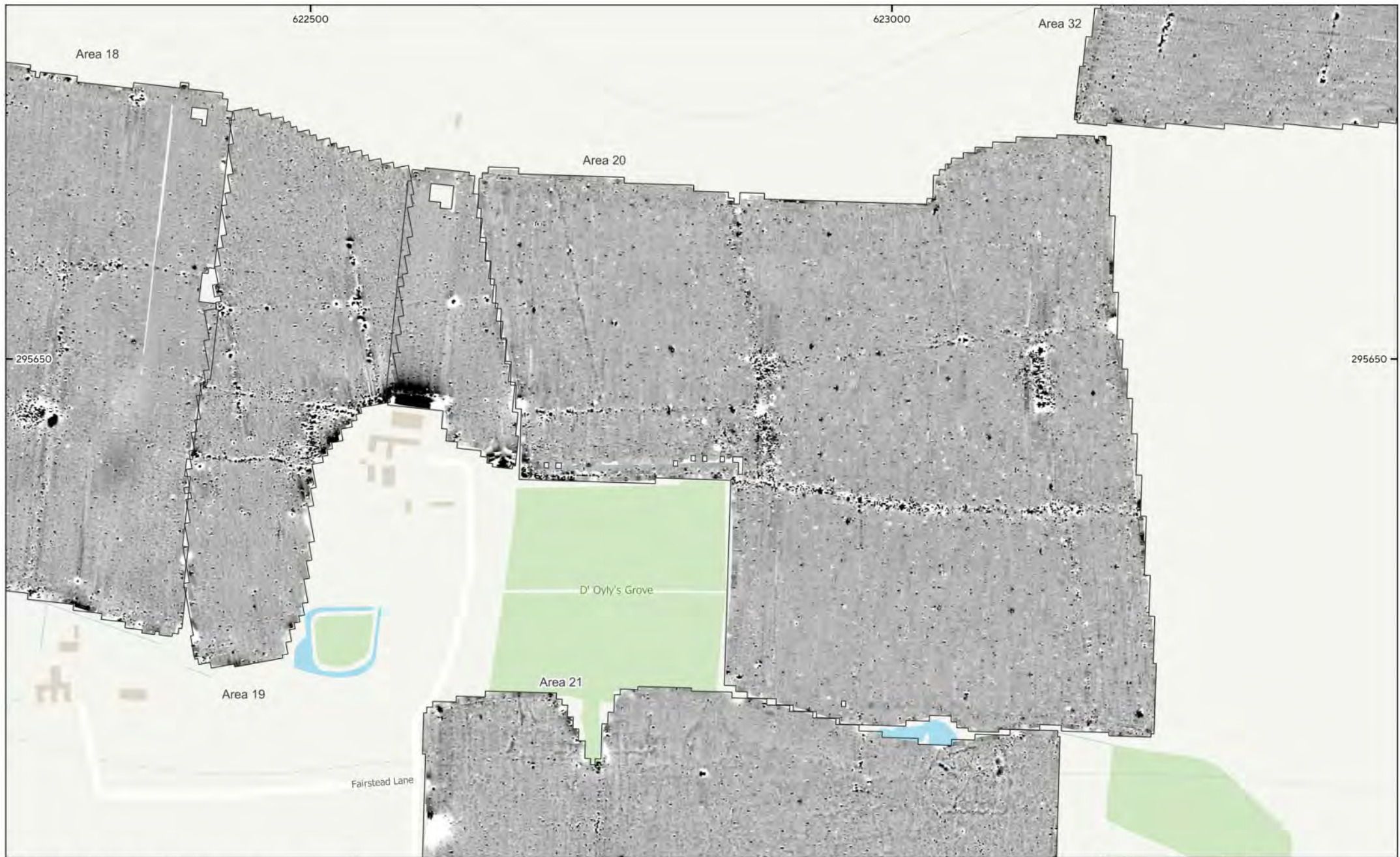
MSTM1774 - East Pye Solar Farm Figure 104 - Magnetic Gradient (Areas 20, 21 & 32) 1:3,000 @ A3 © Magnitude Surveys 2025 Contains Ordnance Survey data © Crown Copyright and database right 2025
