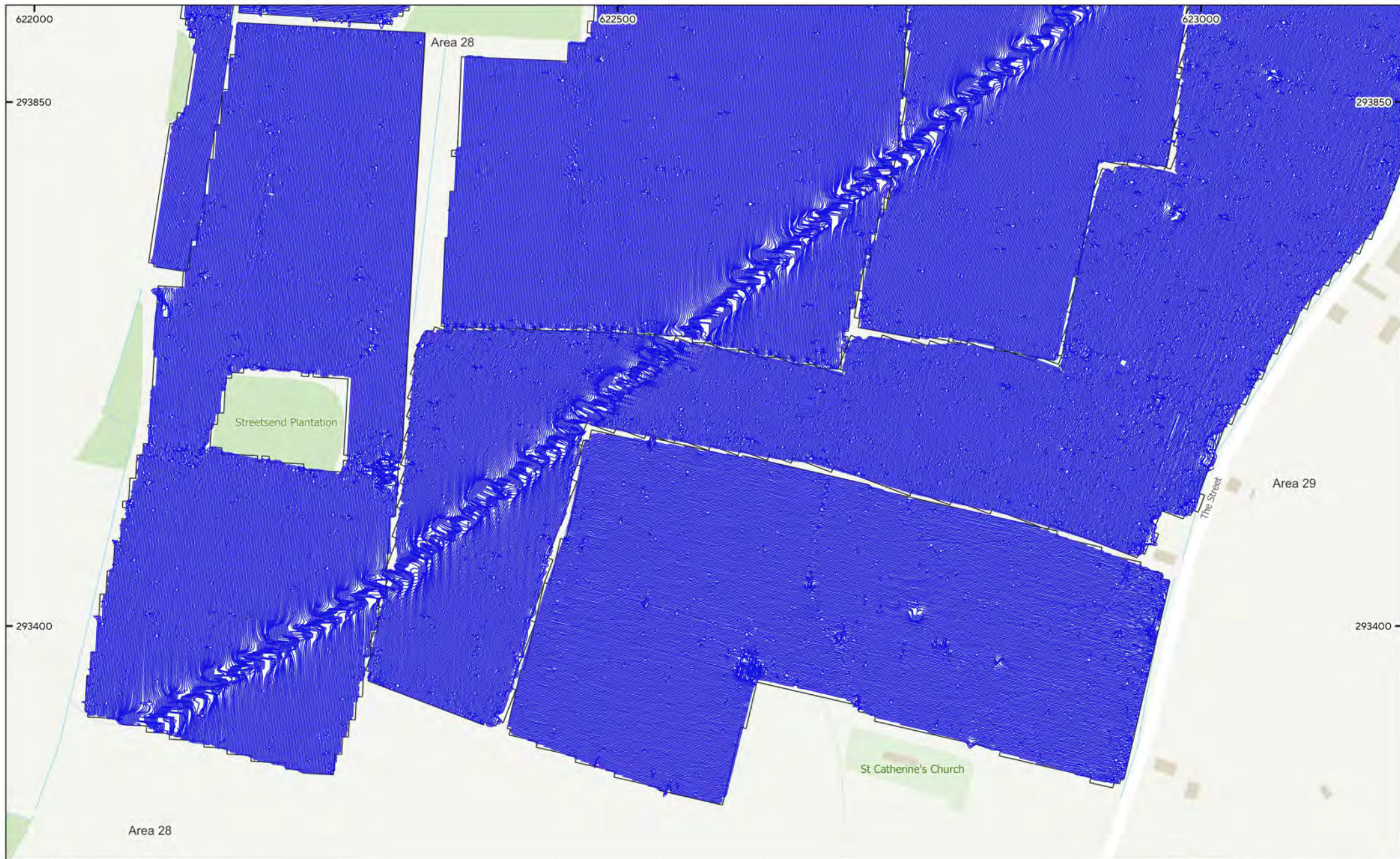
MSTM1774 - East Pye Solar Farm Figure 118 - XY Plot (Areas 25, 26 & 28 to 30) 180nT/cm at 1:3,000 @ A3 © Magnitude Surveys 2025 Contains Ordnance Survey data © Crown Copyright and database right 2025
